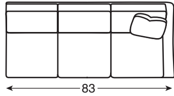
ESN202-52 | RAF Sofa W83 D37 H35 Seat: H20 Arm: H23
