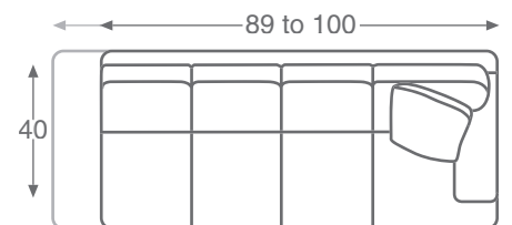
20-22 RAF Sofa W 89-100 D 40 H 37
