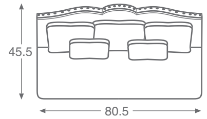
55-788 Center Section Overall W 80.5 D 45.5 H 44.5 Inside W 69 D 20 H 23.5 Seat Height 21
